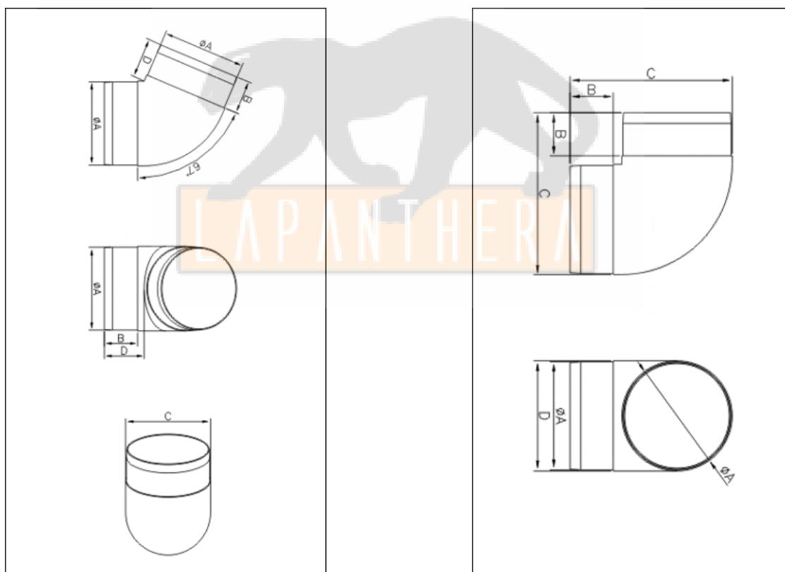
D/KO Ø100/67°
